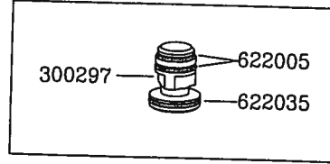
300314 CPL VALVE PISTON
